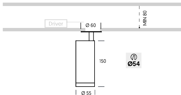
ZOOM 55 SEMIRECESSED
