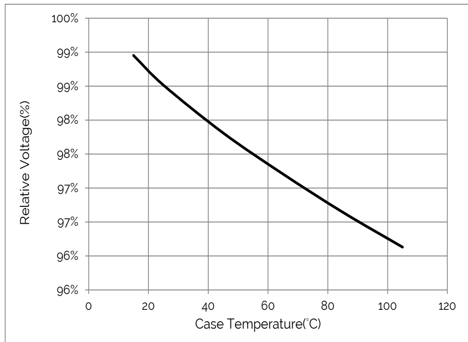
Figure 10: Relative Voltage vs. Case Temperature
