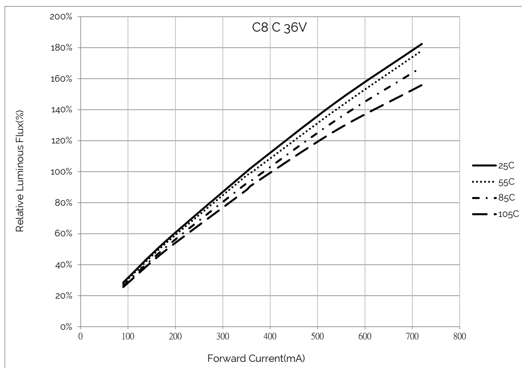
Figure 8: Relative Luminous Flux vs. Drive Current
