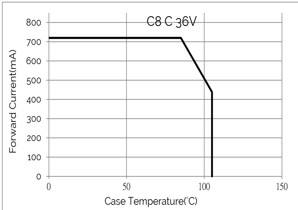
Figure 18: Operating Limits
