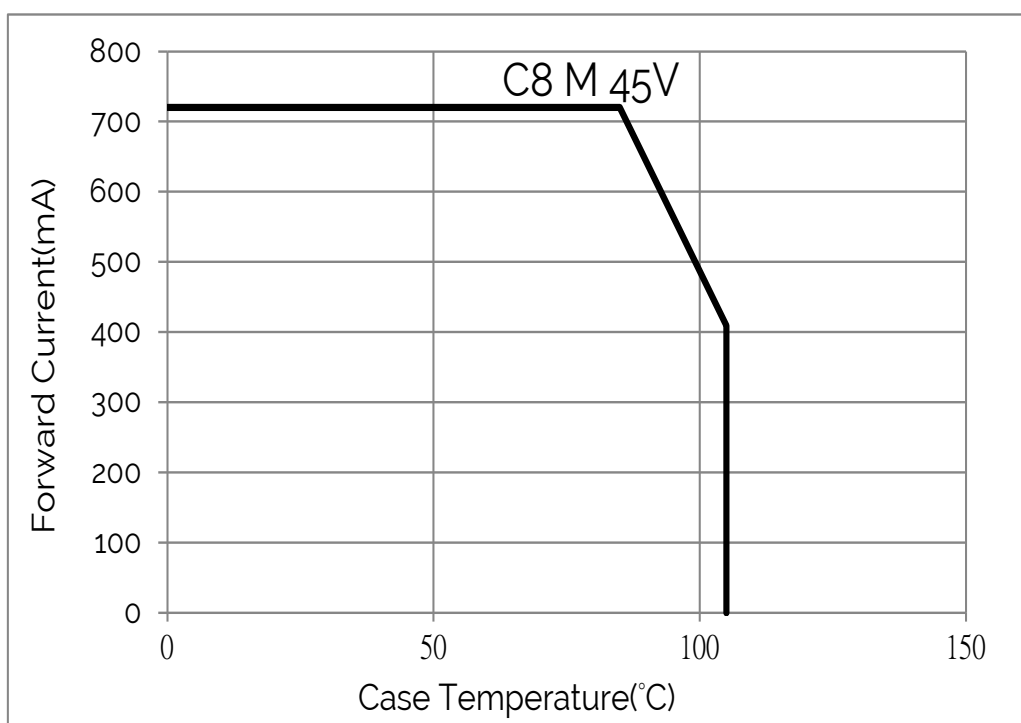
Figure 19: Operating Limits
