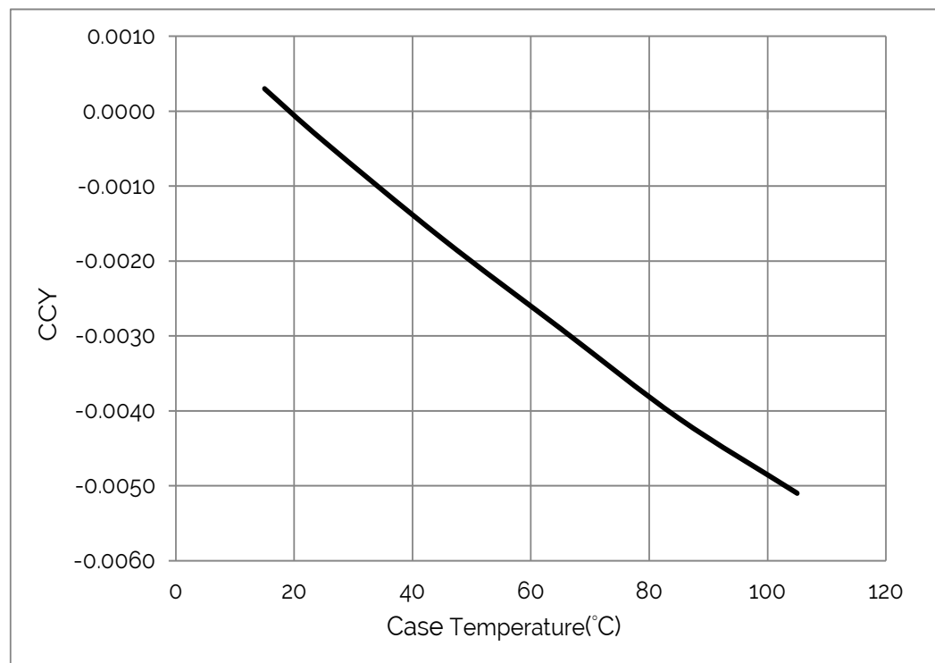
Figure 12: Typical DC ccY Shift vs. Case Temperature
