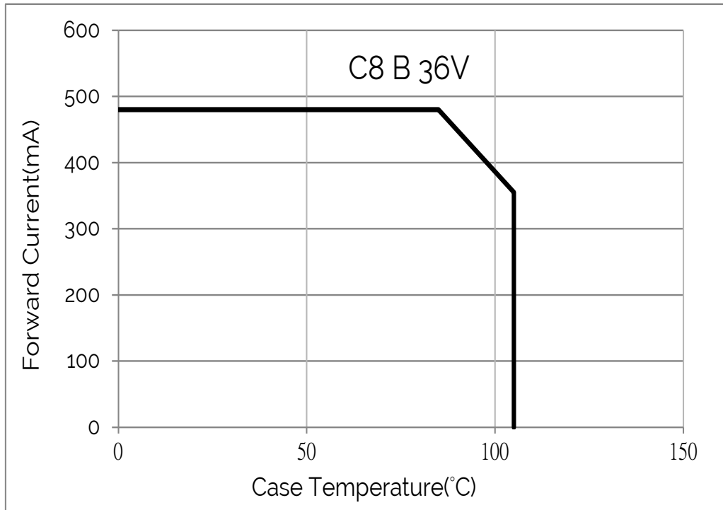
Figure 17: Operating Limits
