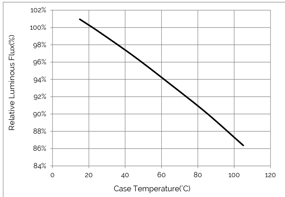
Figure 9: Relative Luminous Flux vs. Case Temperature
